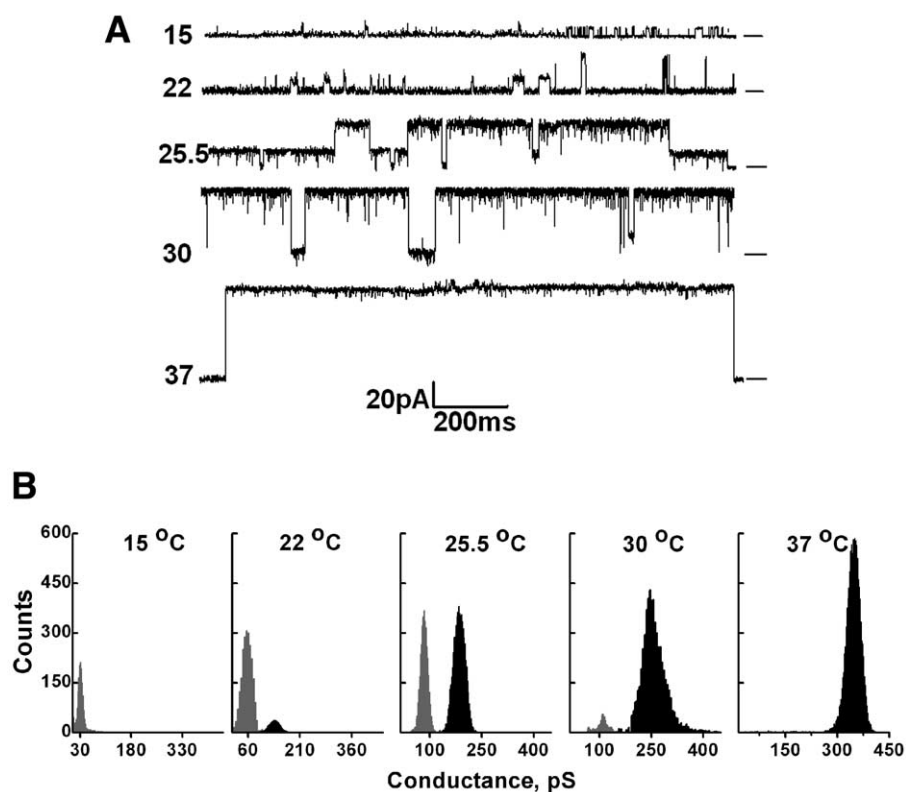
Fig. 1. A: Representative single-channel recordings for OmpA. Protein (ca. 0.2 \mu\text{g} ) in C8E4 was incorporated in planar lipid bilayers formed from DPhPC/ n -decane, between symmetric bathing solutions of 1 M KCl in 10 mM Tris–Cl buffer, pH 7.1. Clamping potential was +100 mV with respect to ground ( trans ). Data were filtered at 1 kHz. The temperature of the chambers was controlled by pyroelectric controller (see Section 2). The temperature in the trans bath (ground) was read directly using a thermoelectric junction thermometer which also served as a point of reference for the pyroelectric controller. Temperatures are indicated on the left hand side of each trace, and the closed state is delineated by a horizontal bar at the right side of each trace. B: The corresponding amplitude histograms showing the distribution of small (gray) and large (black) OmpA channels at increasing temperatures. The closed state is not shown.
